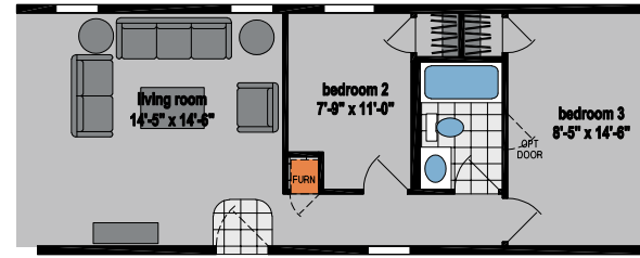
ALTERNATE FRONT BEDROOM/HALL BATH
