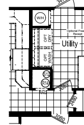
Ceiling Duct w/o Furnace
